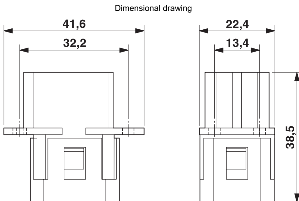
HC-COM-8-EBUC dimensional drawing
