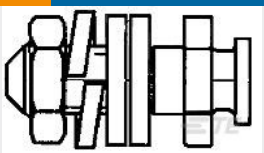
TE Part # 5206514-1 SLIDING LOCK POST KIT
