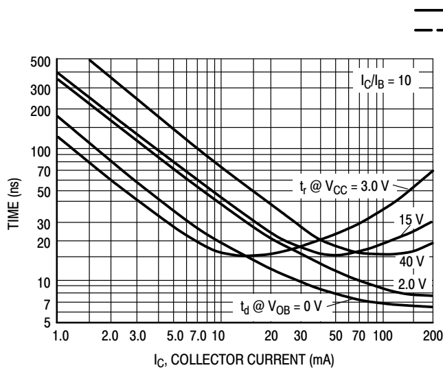
Figure 4. Turn - On Time
