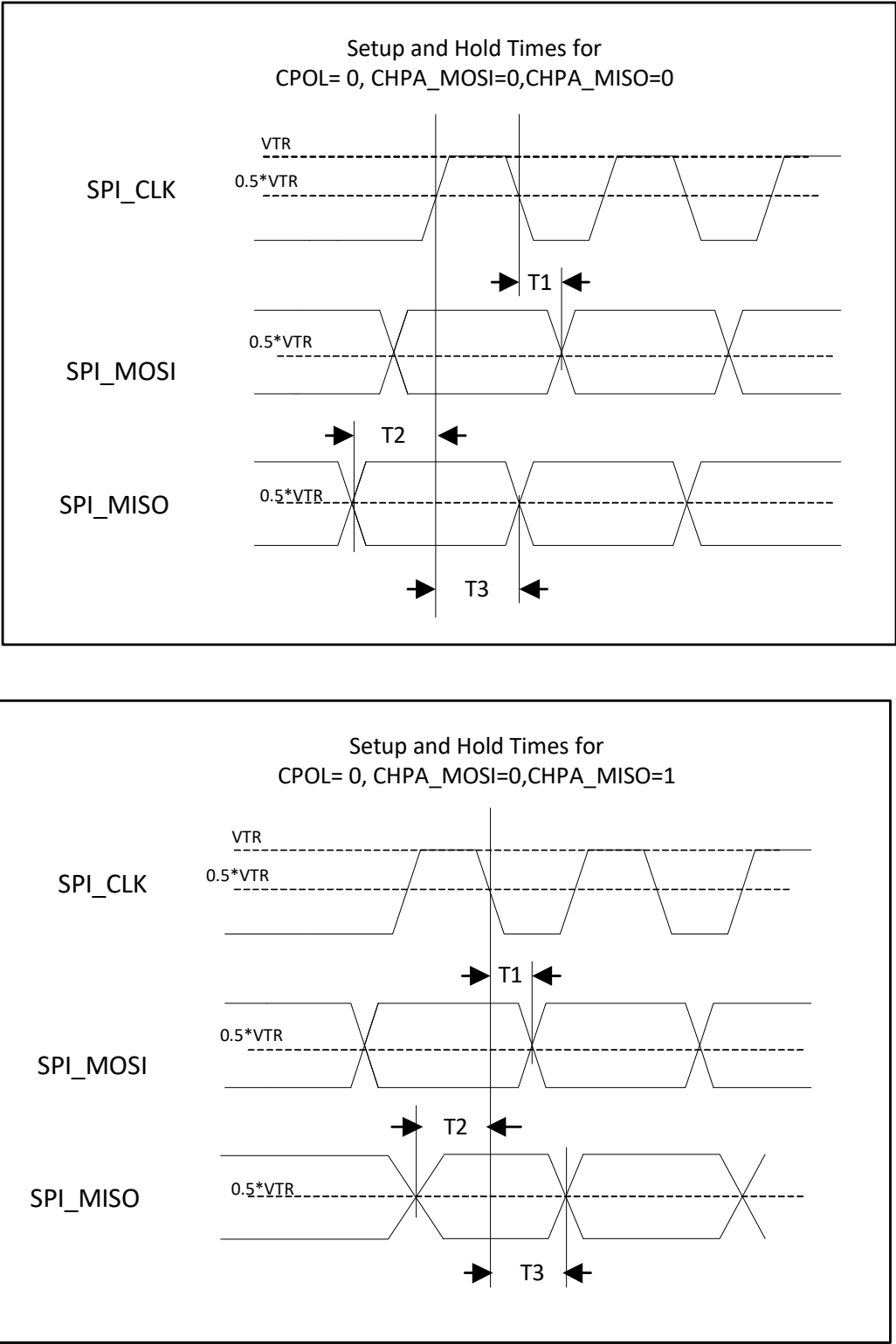
FIGURE 34-12: SPI SETUP AND HOLD TIMES
