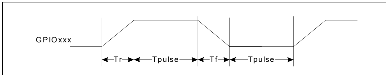
FIGURE 34-5: GPIO TIMING
