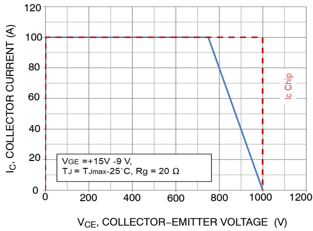
Figure 26. RBSOA
