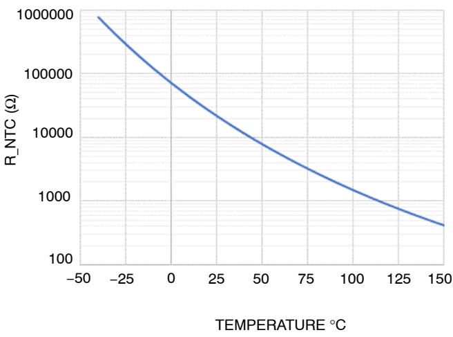
Figure 29. Temperature vs NTC Value
