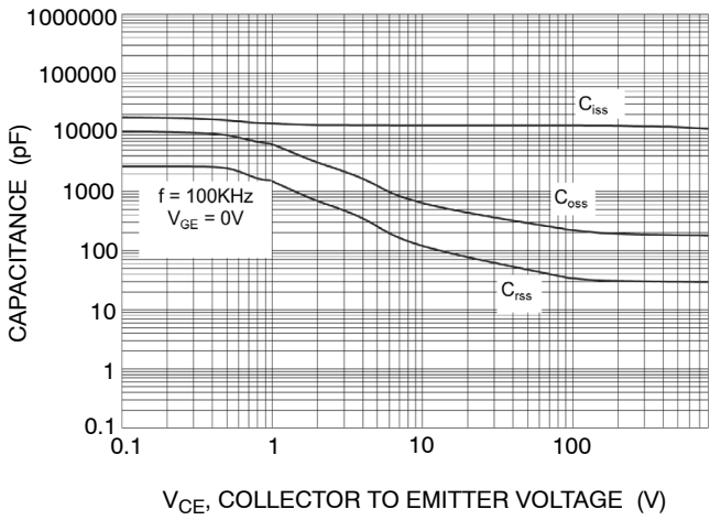
Figure 27. Capacitance Charge
