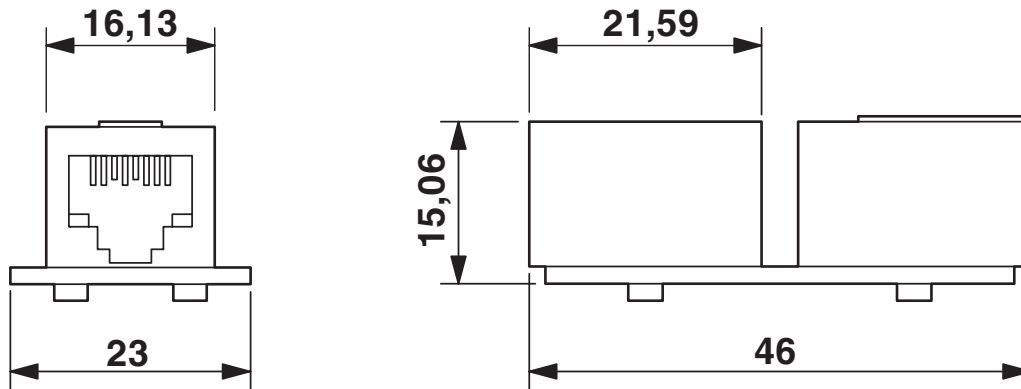
Dimensional drawing
