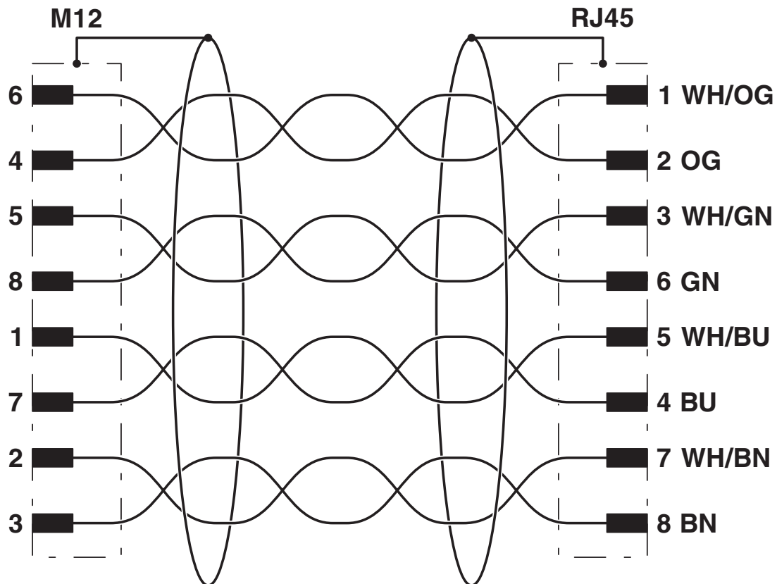
Circuit diagram
