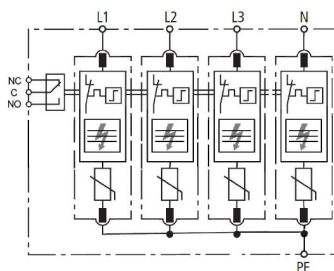
Three-phase wye (star) four-wire+ground
