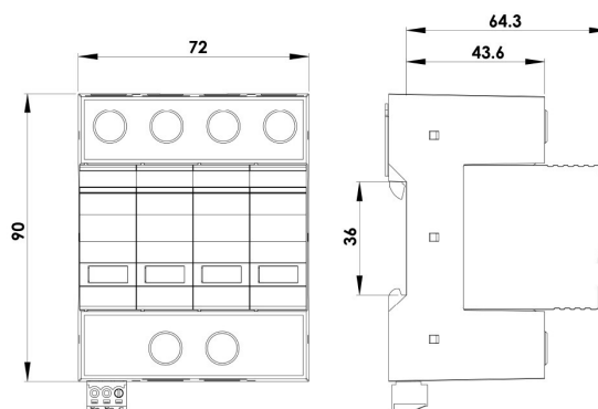
4Pole (72mm width)
