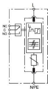
Single-phase two-wire
