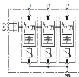
Three-phase delta /wye three-wire+ground
