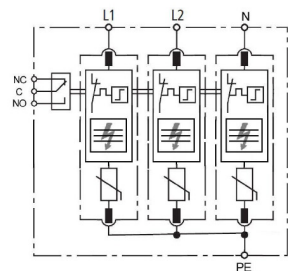
Split-phase three-wire+ground
