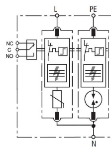
Single-phase two-wire+ground
