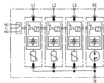
Three-phase wye (star) four-wire+ground
