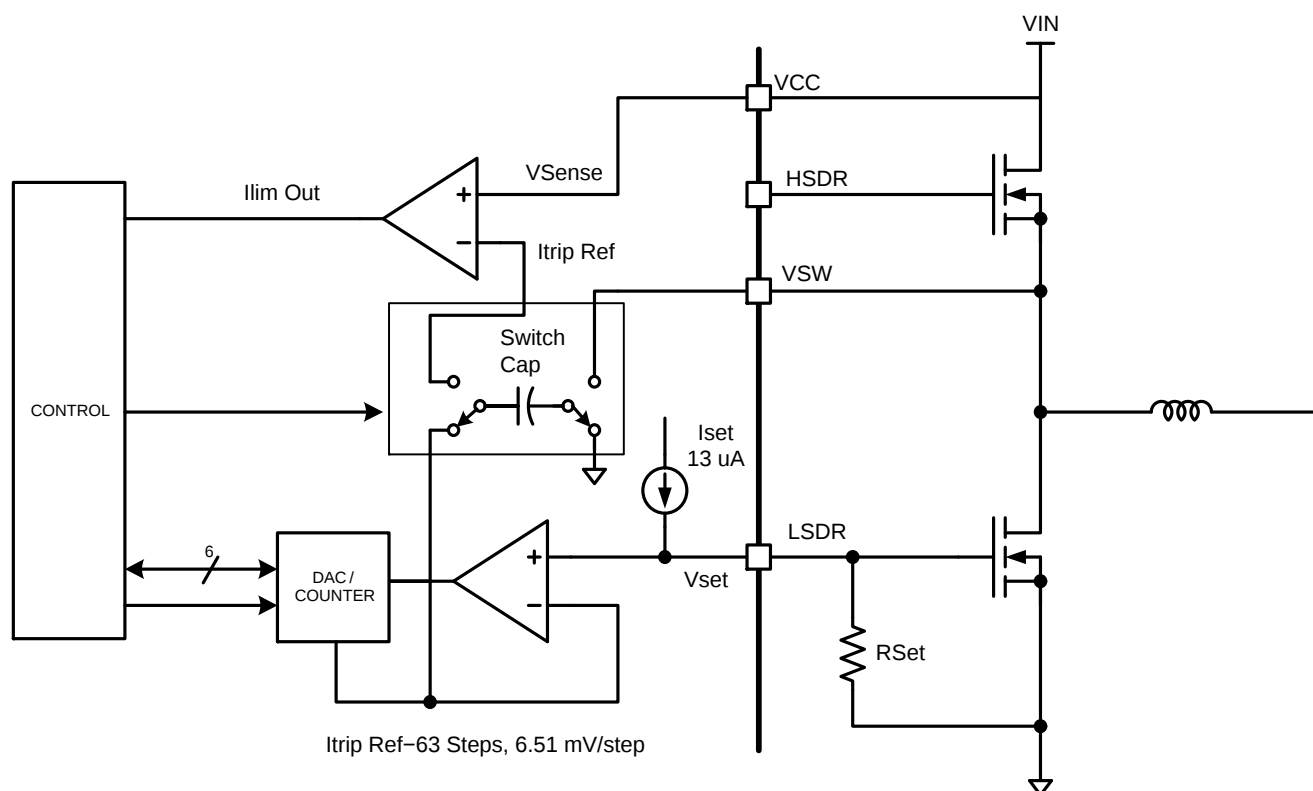
Figure 36. I_{\text{set}} / I_{\text{Limit}} Block Diagram
