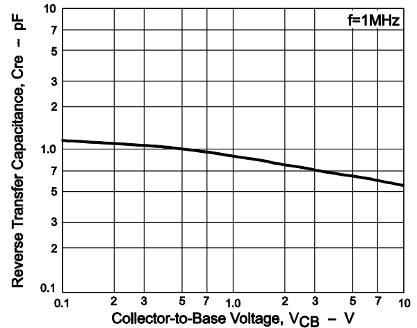
Figure 6. C_{re} - V_{CB}
