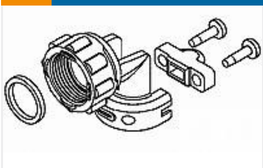
TE Part # 796381-2 R/A STRN RELIEF KIT,SZ 17,CPC
