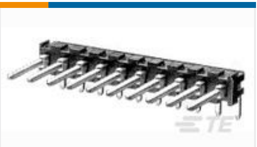
TE Part # 87232-2 02 MODII HDR SRRA UNSHRD .100
