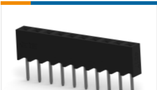
TE Part # 1-2314878-0 10P,2MM,B-B,REC,SRVT,2.7,0.76AU,TB
