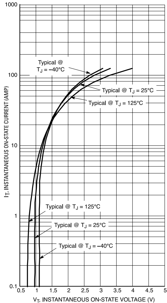
Figure 3. On-State Characteristics
