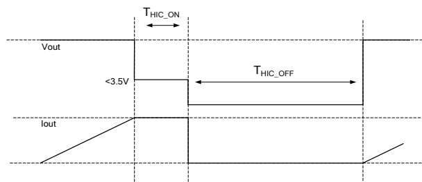
Figure 7: Over-Current Protection
