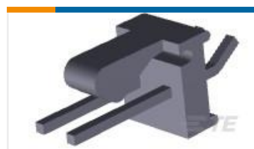
TE Part # 644874-2 02P MTA100 HDR ASSY, SPCL BEND
