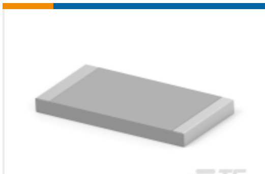
TE Part # 4-2176331-8 CRGP 2512 82K 1%
