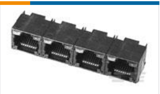
TE Part # 5557562-1 MOD JK ASSY,4PORT,8POSN,RTANG
