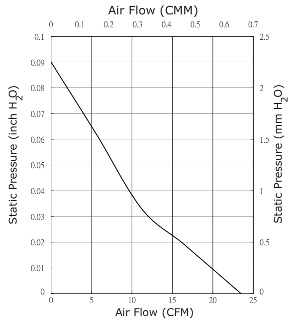
CFM-7020V-232-330
