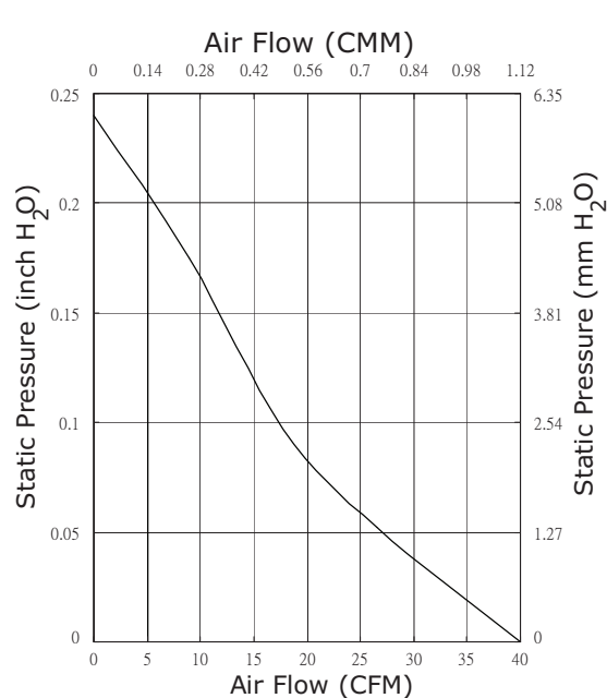
CFM-7020V-143-400
