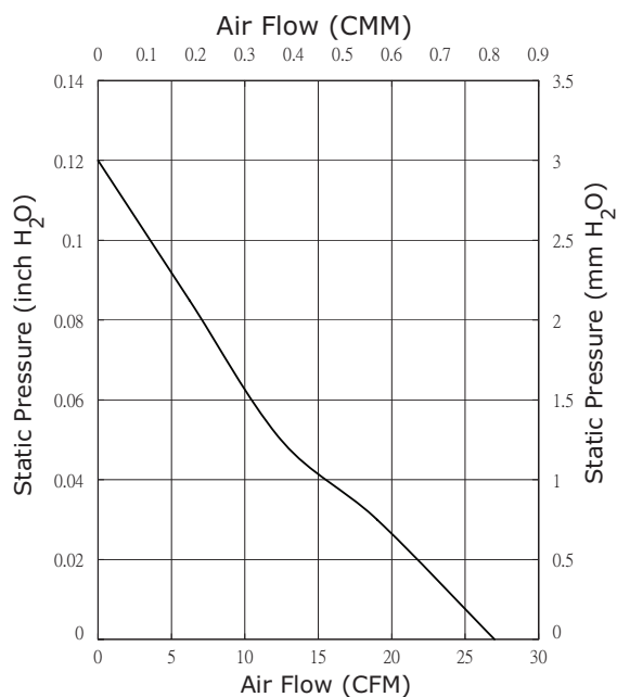
CFM-7020V-140-375
