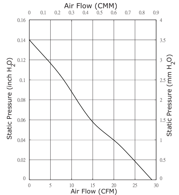
CFM-7020V-232-330
