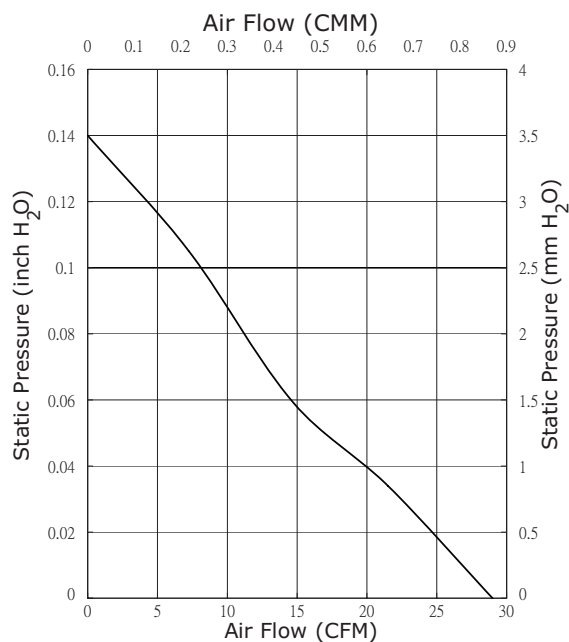
CFM-7020V-143-400
