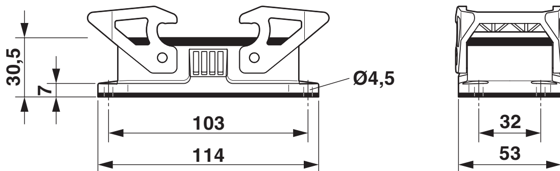
Dimensional drawing
