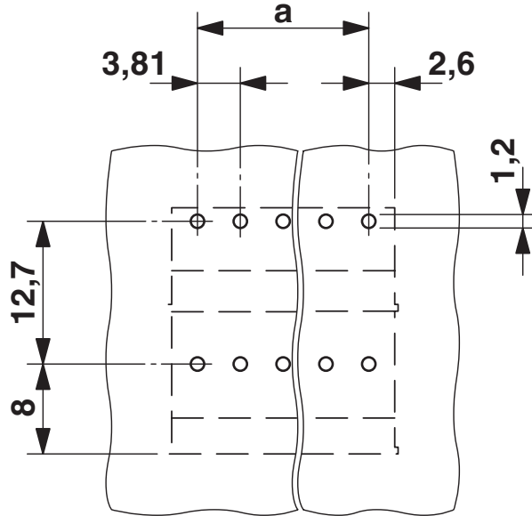
Dimensional drawing
