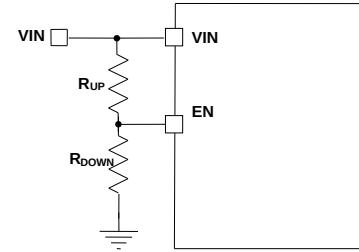
Figure 5: Adjustable UVLO Using EN Divider
