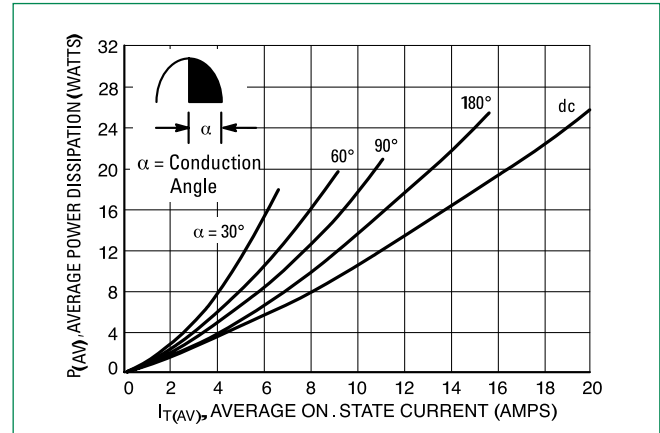
Figure 8. On State Power Dissipation
