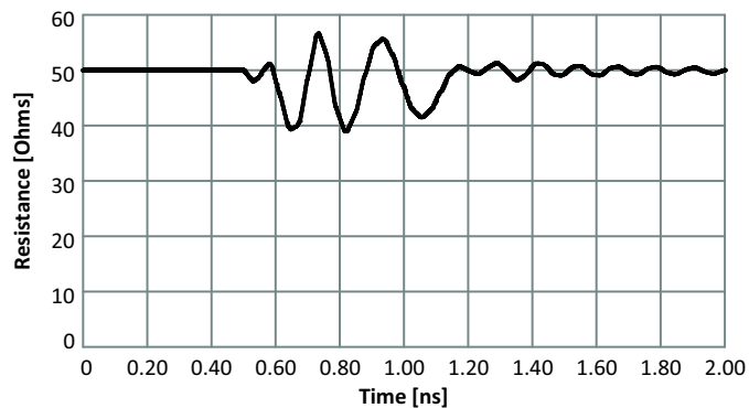
Figure 16. TDR - ESD8040
