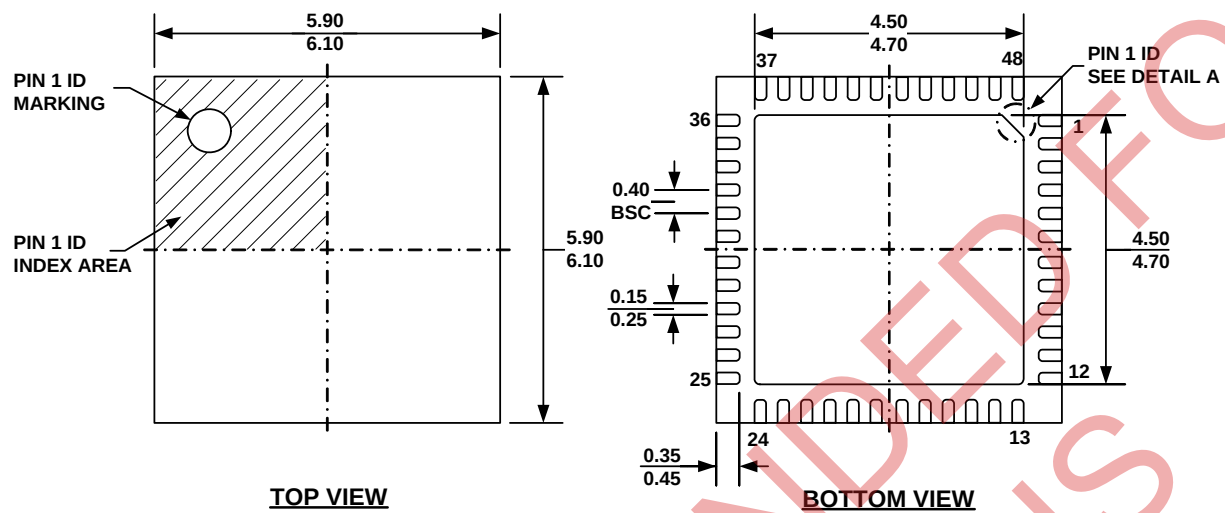
QFN48 (6 x 6mm)
