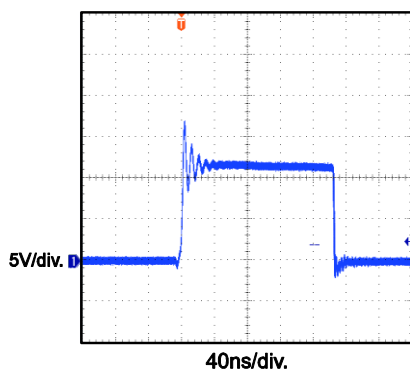
SW Output Waveform
