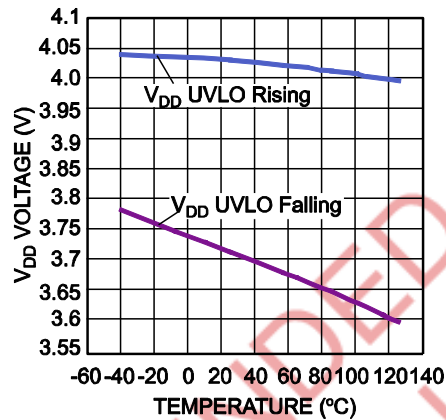
V_{DD} UVLO Threshold vs. Temperature
