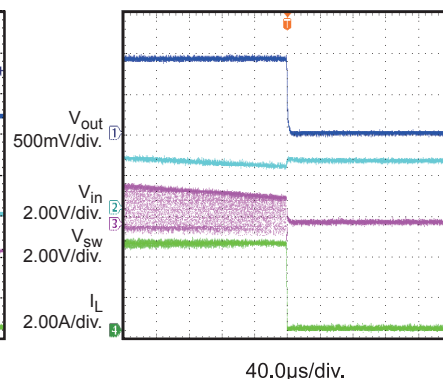
VIN Shut Down with 2A Load
