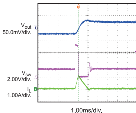
Output Ripple
