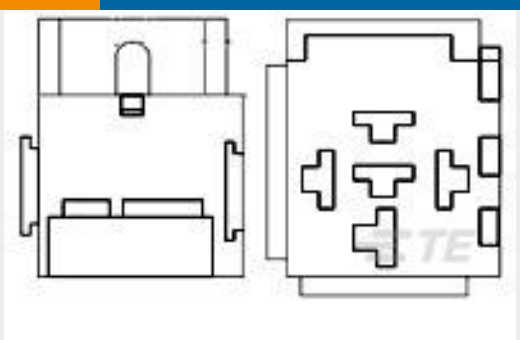
TE Part # 4-1419106-0 VCF4-1002=CONNECTOR,HOUSING-
