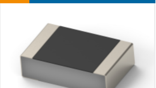
TE Part # 5-2176453-3 CPF 0201 20K 0.1% 25ppm 1K RL
