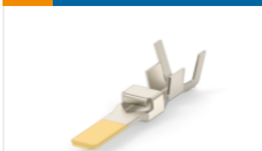
TE Part # 917803-3 Contact: Component To Wire ; 20-45A , 20-8 wire size
