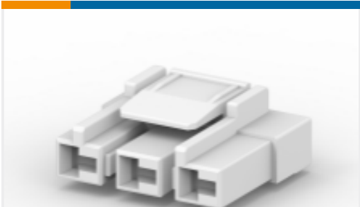
TE Part # 1903414-2 GHC 9.0 3POS PLUG HSG
