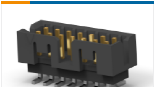
TE Part # 1-2842244-4 14P,2MM,SHRD HDR,DRVT,SMD,0.1 AU,TB W/CP
