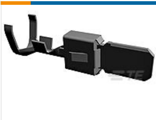
TE Part # 964312-1 TAB A 5.8x0.8 CONTACT CF SWS Sn
