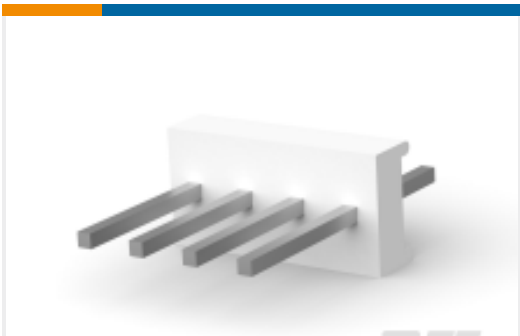
TE Part # 640456-7 PCB Header: Polyester, Vertical, Unshrouded, No Mating Alignment
