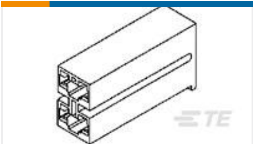
TE Part # 172210-1 POSITIVE LOCK 250 HOUSING RECEPTACLE
