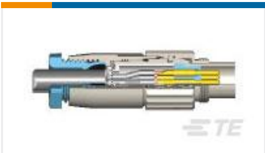
TE Part # 1-1437719-5 T01-0550-P03-MALE PLUG CONNECTOR SOLDER
