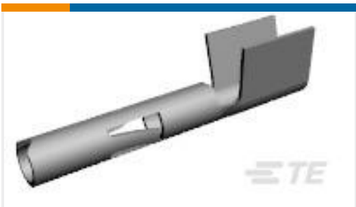
TE Part # 640310-6 UMNL SOK 12-10 AU/PHBZ
