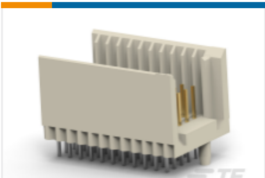
TE Part # 5100141-1 Hard Metric Male Connector: Traditional Backplane, Mezzanine, 2mm
