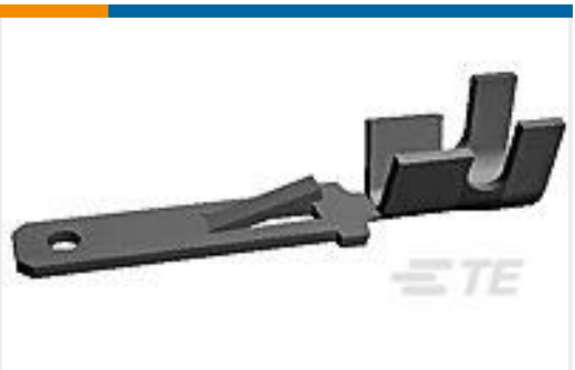
TE Part # 42098-1 FF 250 TAB 18-14 AWG .032 BR
