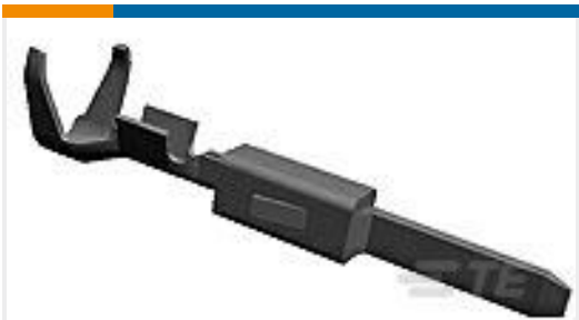
TE Part # 964270-2 TAB A 1.6x0.6 CONTACT CF SWS Sn (LP)
