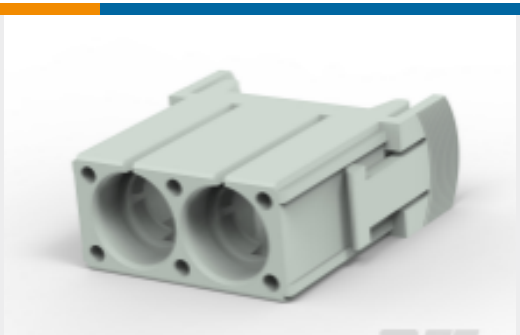
TE Part # T2111022301-000 HMN-PA2
