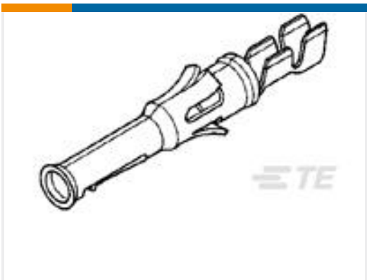
TE Part # 66594-4 TYPE VI SKT,MULTI-MATE,L.P.
