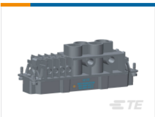
TE Part # T2100122101-000 HK4/8-012-M
