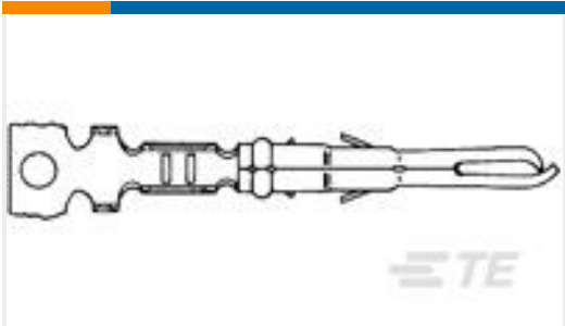
TE Part # 640545-1 MR SPLIT PIN 26-18 PTPHBRZ LP
