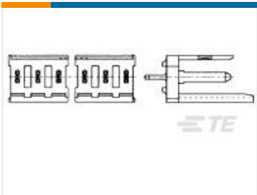
TE Part # 280611-2 6P MOD 1 SHROUDED HEADER, ST, 0.4 Au
