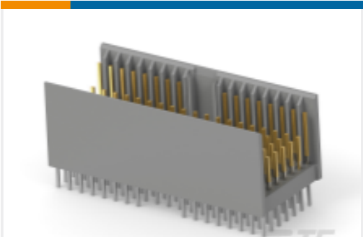
TE Part # 5646530-1 Z-PACK 2MM HM TYPE A/B 127P
