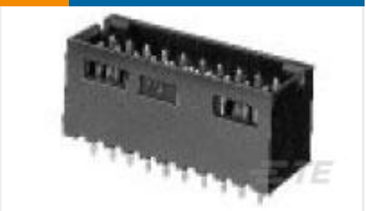
TE Part # 6-102618-5 34 MODII HDR DRST SHRD .100CL
