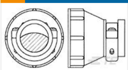
TE Part # 182930-1 CPC Cable Clamp Kit, Size 23, Large, UV
