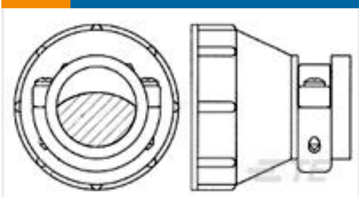
TE Part # 182661-1 CPC Cable Clamp Kit, Size 17, Large, UV
