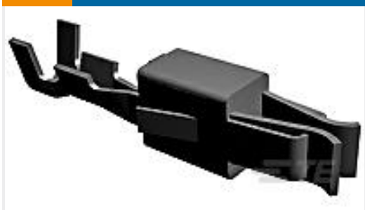
TE Part # 927779-6 JPT REC 2.8 Contact SRC Ag (LP)
