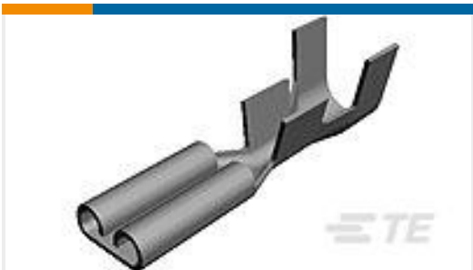
TE Part # 42566-2 187 FASTON REC 20-16 AWG TPBR
