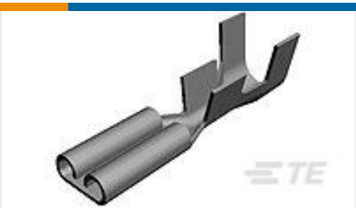
TE Part # 42067-1 110 FATON REC 24-22 AWG TPBR
