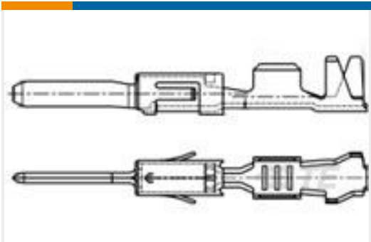
TE Part # 963900-1 TAB A 1.6x0.6 CONTACT CS SRC Sn
