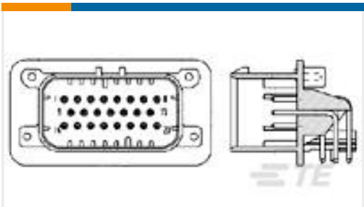
TE Part # 776087-1 23POS,PIN DIA 1.3,HDR ASSY,90DEG, COD 1
